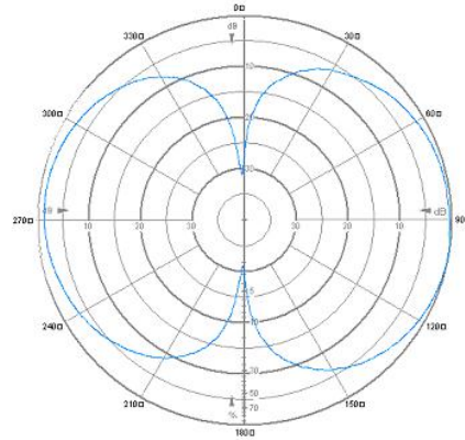
Vertical pattern
